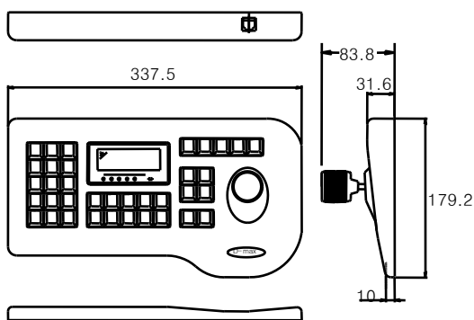
KEYBOARD
