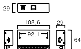
JUNCTION BOX
